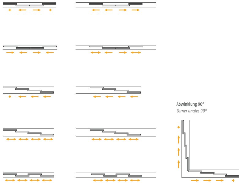
Standard-Laufschiene Standard track slide
